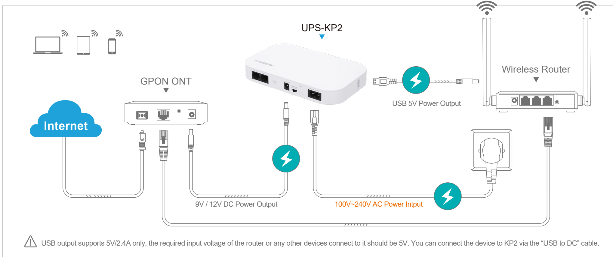
Typical topology 3: Powering up 2*DC devices
