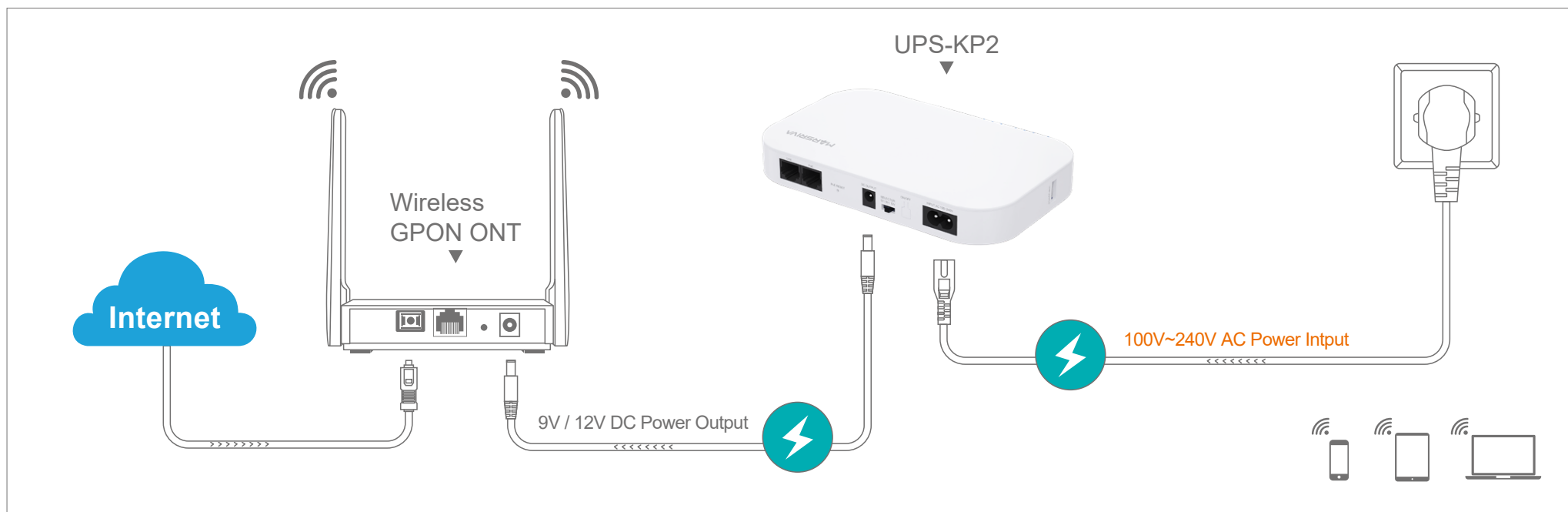
Typical topology 2: Powering up 1*DC device
